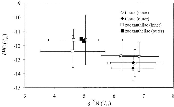
Fig. 4. Mean \delta^{13}\text{C} and \delta^{15}\text{N} of coral tissue from all sites. Note the absence of significant differences in the \delta^{13}\text{C} and \delta^{15}\text{N} between the inner and out reef sites.
