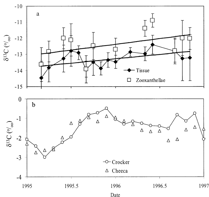
Fig. 2. (a) Changes in the \delta^{13}\text{C} of the coral tissues and the zooxanthellae over the time period January 1995 to December 1996. There is an increase in the \delta^{13}\text{C} of both the zooxanthellae ( r^2 = 0.10 ) and the coral tissue ( r^2 = 0.29 ) over this time period. The change in the \delta^{13}\text{C} of the coral tissues is statistically significant at the 95% level ( p < 0.05 , n = 16 ). (b) Changes in the \delta^{13}\text{C} of the coral skeleton of M. faveolata collected from Crocker Reef and S. siderea collected from Cheeca Rocks over the same time period as measurement of the \delta^{13}\text{C} of the coral tissue and zooxanthellae. These two records both exhibit a small increase during the experimental period superimposed on an overall decrease in the \delta^{13}\text{C} of the skeleton as a result of the ^{13}\text{C} Suess effect (see Fig. 7). Data measured on zooxanthellae from December 1995 and March 1996 have been omitted for scaling reasons (see Table 1).
