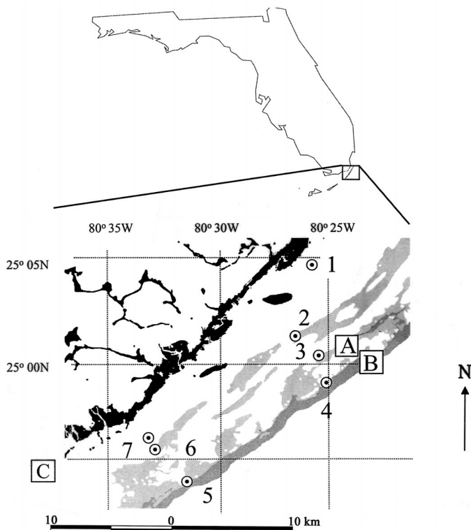
Fig. 1. Location of the reefs studied in the Florida Keys. Site 2 (triangles), site 4 (Pickles), site 5 (Crocker), site 6 (Hen and Chickens), and site 7 (The Rocks). In addition, water samples were collected from marker 2 (site 1) and Molasses Channel (site 3). The location of sites from which water samples are collected for the Florida Keys National Marine Sanctuary (FKNMS) water-quality network are shown in the squares (Molasses Channel (A) and Molasses Reef (B)). The coral skeletons analyzed were collected from Crocker Reef (site 5) and Cheeca Reef (C). The shading denotes 20 ft depth contours. Land and semiemergent mudbanks are shown in the black shading.
