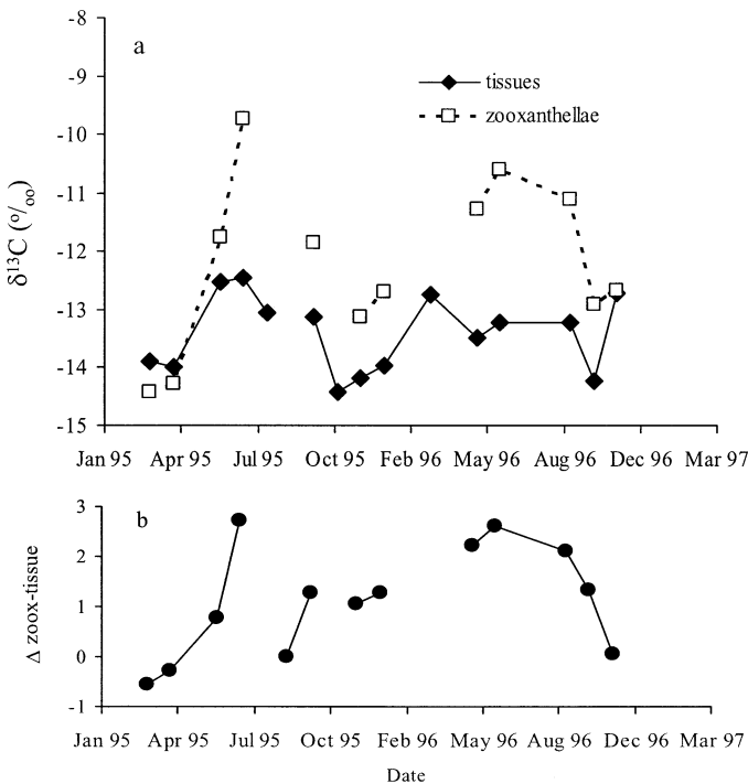
Fig. 5. (a) Seasonal changes in the \delta^{13}\text{C} of the coral tissue and the zooxanthellae in the corals from ~8 m at Pickles Reef. This site show a very clear seasonal change in the \delta^{13}\text{C} of both the fractions as well as a seasonal difference between the \delta^{13}\text{C} of the zooxanthellae and the coral tissue. (b) Changes in the difference between the zooxanthellae with respect to season. Maximum difference between the zooxanthellae and the coral tissue occur during the summer months.
