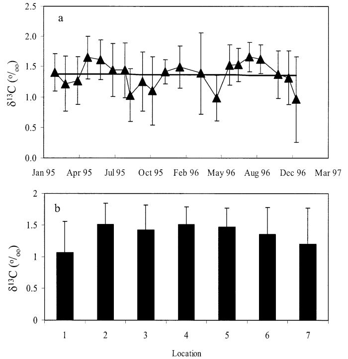
Fig. 6. (a) Changes in the \delta^{13}\text{C} of the DIC at sites shown in Fig. 1. Note that there are only 2 yr worth of data yet there are four cycles in the \delta^{13}\text{C} DIC data. These multiple changes also appear to be present in the \delta^{13}\text{C} signal in the coral skeleton. (b) The mean and standard deviation (error bars) of the \delta^{13}\text{C} of the DIC from all seven sites studied during this investigation are shown.
