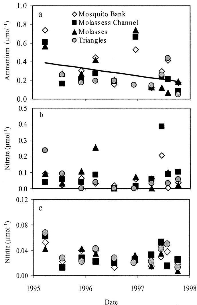
Fig. 7. Changes in the concentration of (a) \text{NH}_4^+ , (b) \text{NO}_3^- , and (c) \text{NO}_2^- from locations near the collection sites of the coral tissue during the time period of the study (data are from FIU-SERC). The trend line in (a) shows the decrease in the concentration of \text{NH}_4^+ at Molasses Reef. Although the decrease is not statistically significant at the 95% confidence limits ( r^2 = 0.13 , n = 10 ), the change mirrors decreases in the \delta^{15}\text{N} of the coral tissues over the same time period.
