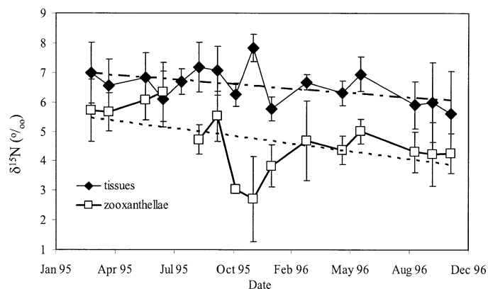
Fig. 3. Changes in the \delta^{15}\text{N} of the coral tissues and the zooxanthellae over the time period January 1995 to December 1996. There is a statistically significant decrease in the \delta^{15}\text{N} of both the zooxanthellae and the coral tissue. The r^2 of the coral tissue and the zooxanthellae are 0.25 ( n = 16 ) and 0.34 ( n = 14 ), respectively.
